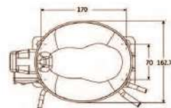
WD 系列外形图 Outline of WD series compressors
